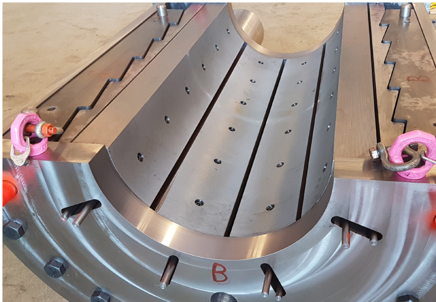
01 // Large surface area gripping system used to transfer loads
